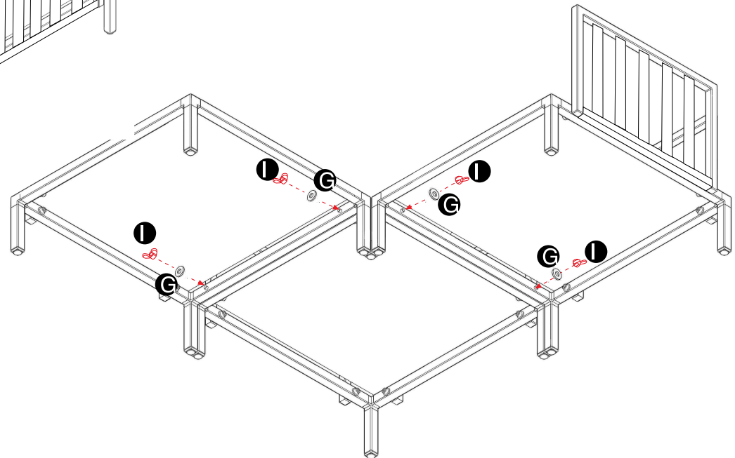
BOTTOM VIEW
